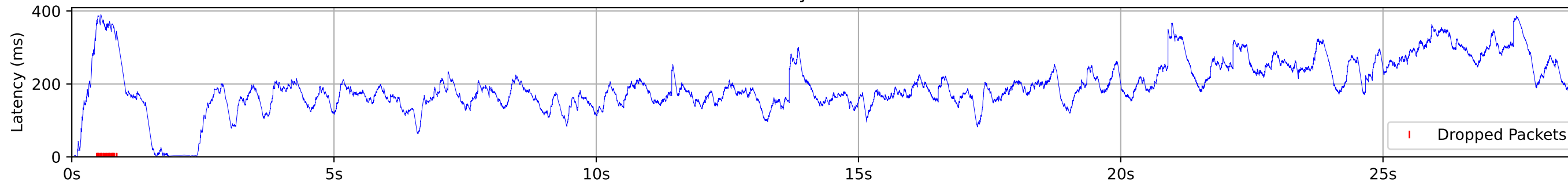
Latency Timeseries
