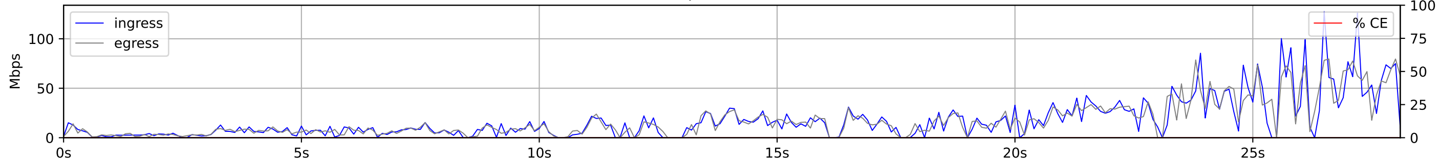
Mbps Timeseries
