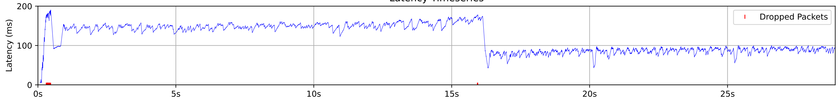
Latency Timeseries
