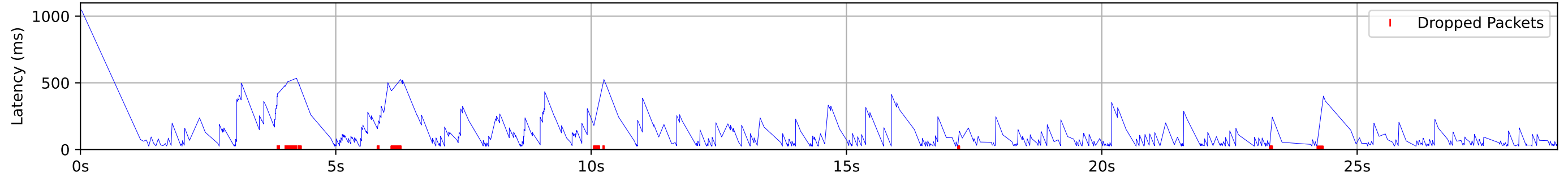
Latency Timeseries
