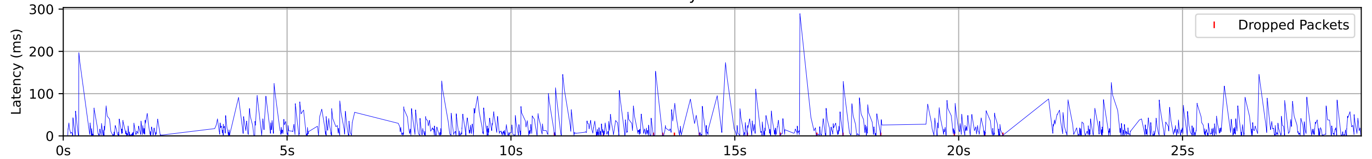
Latency Timeseries
