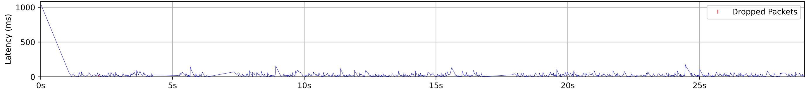
Latency Timeseries
