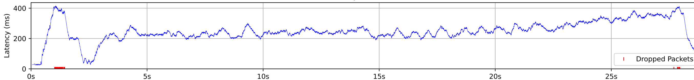
Latency Timeseries
