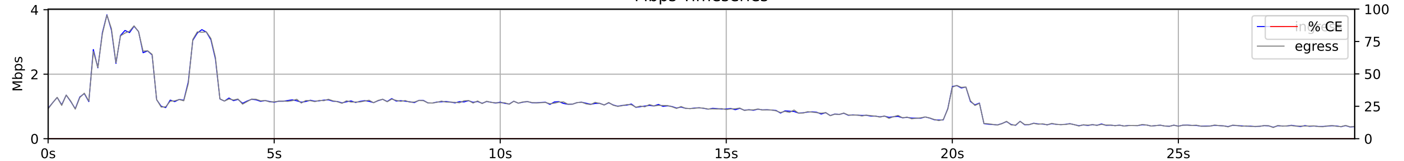
Mbps Timeseries
