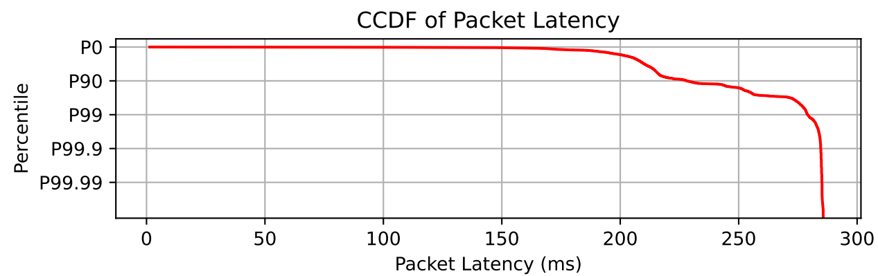
Packet Delay Statistics
