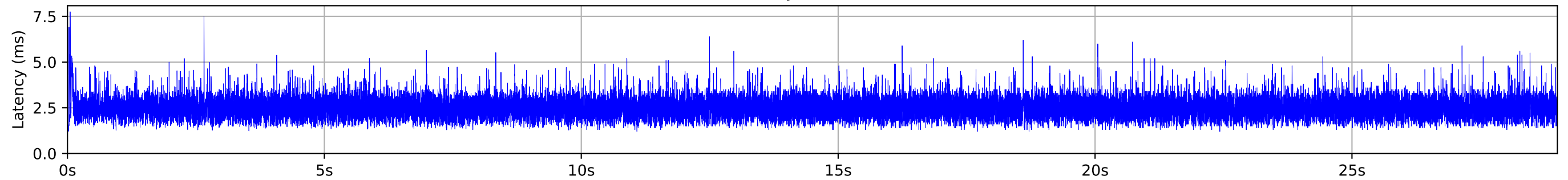
Latency Timeseries
