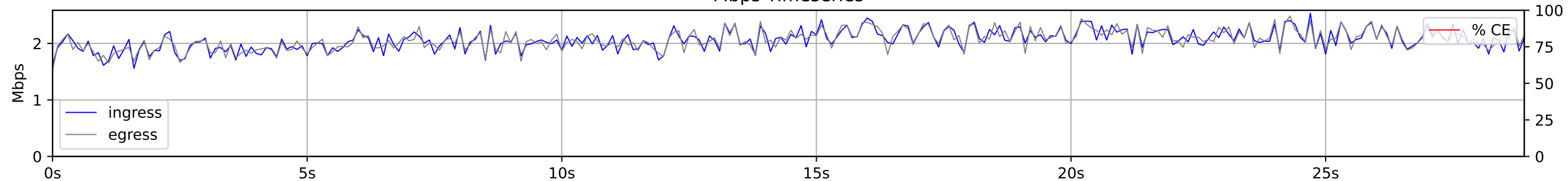
Mbps Timeseries
