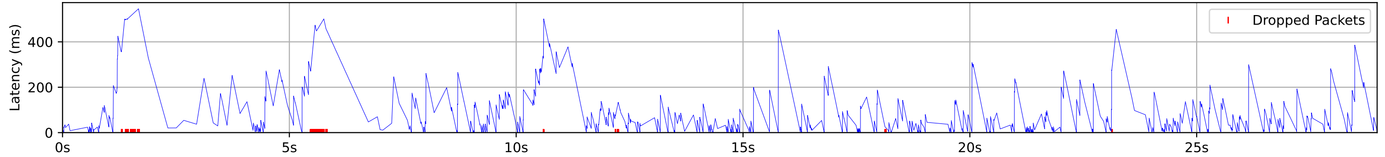
Latency Timeseries
