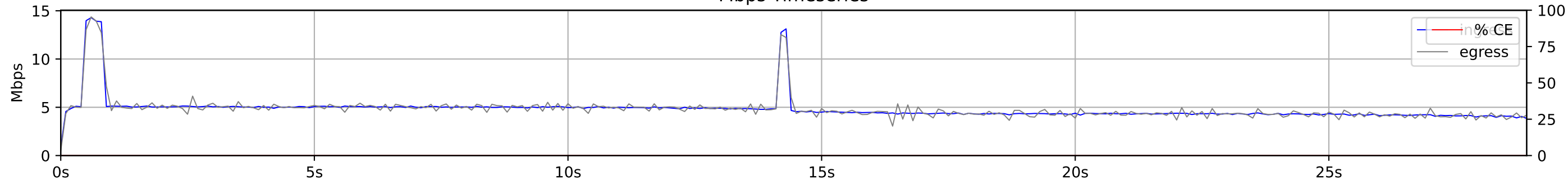
Mbps Timeseries
