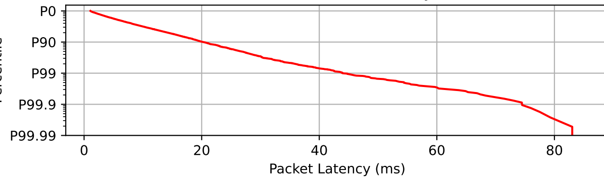
CCDF of Packet Latency
