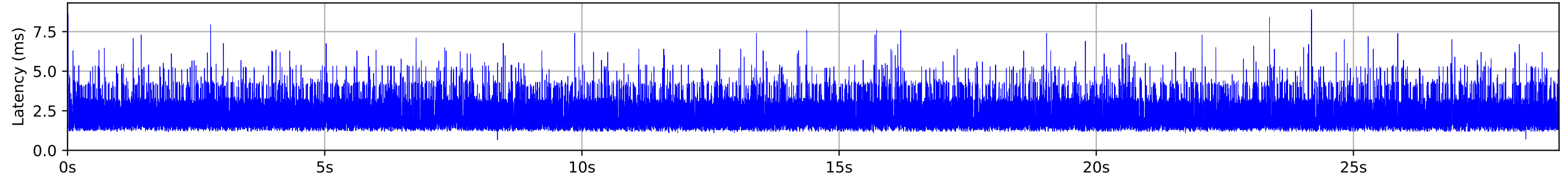
Latency Timeseries
