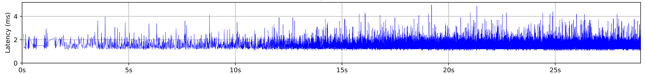
Latency Timeseries
