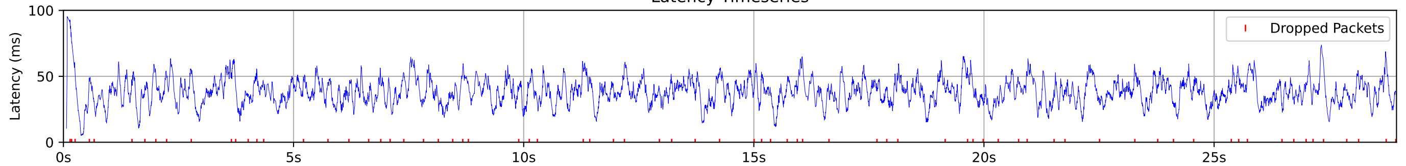
Latency Timeseries
