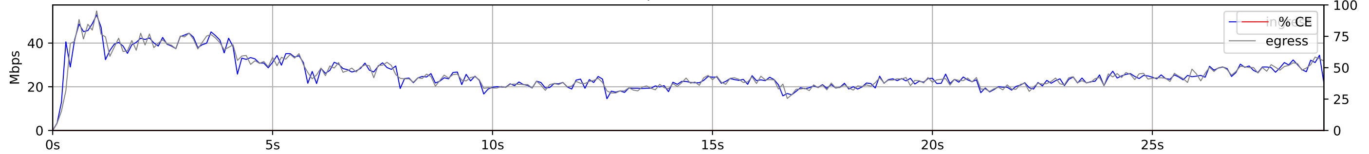
Mbps Timeseries
